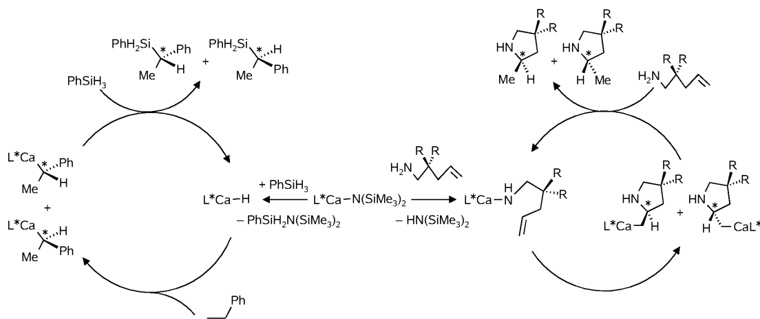
Scheme 2. Catalytic hydrosilylation (left) and hydroamination (right); L* represents the chiral ligand.
