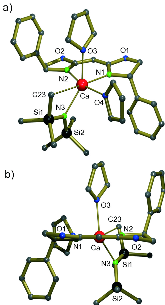
Fig. 1. (a) Crystal structure of [(S)\text{-Ph-BOX}]\text{CaN}(\text{SiMe}_3)_2 \cdot (\text{THF})_2 ( 9 ); hydrogen atoms omitted for clarity. Selected bond lengths and angles are given in Table 1. (b) View along the approximate C_2 axis of the BOX ligand.
